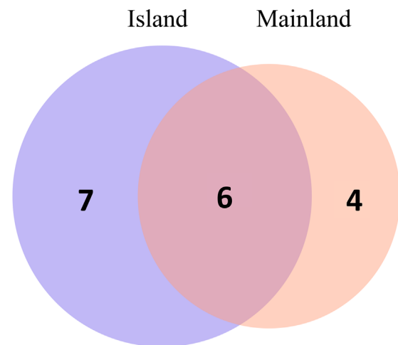
B – Venn diagram for elasmobranchs
