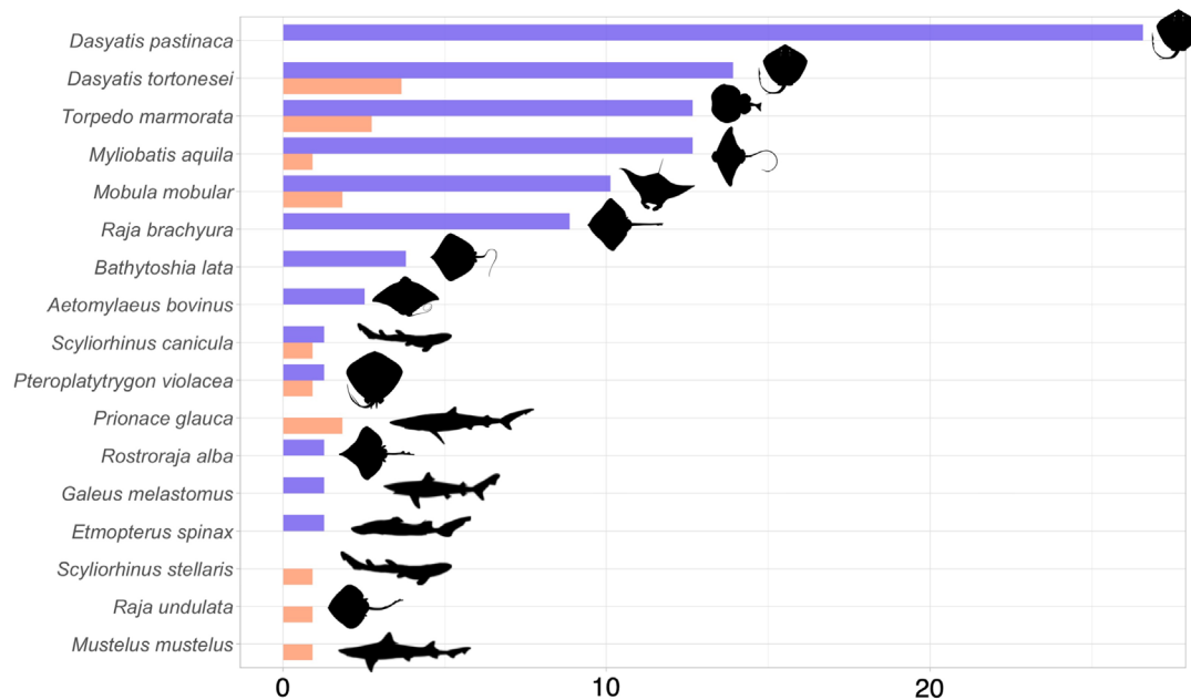
FIGURE 2 | Teleost and elasmobranch species detected using eDNA metabarcoding in 187 eDNA samples along North-Western Mediterranean coasts. The Venn diagrams show species richness overlap between continental and island coastline samples for all fish species (A) and for elasmobranch species specifically (B). Horizontal barplots display the relative frequencies of each elasmobranch species across samples in the two sets of locations (C).
